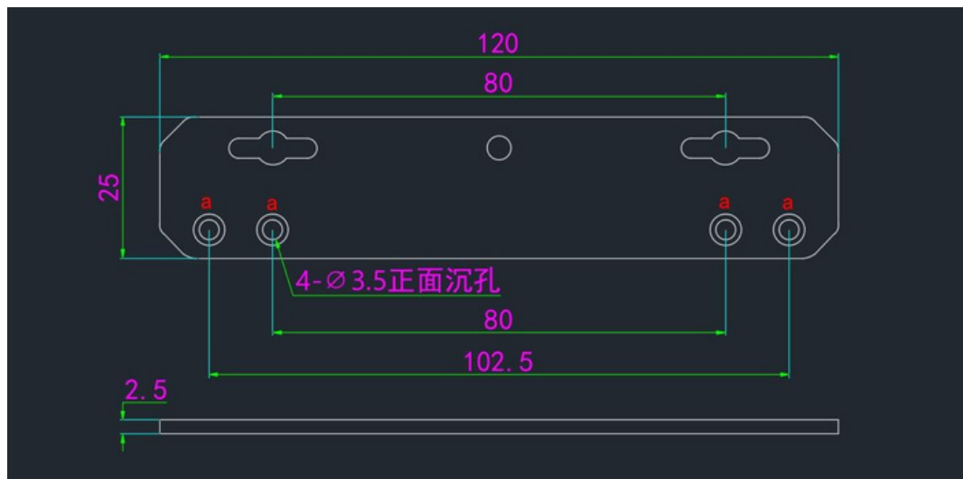
AXBOX-M422 wall mount bracket
