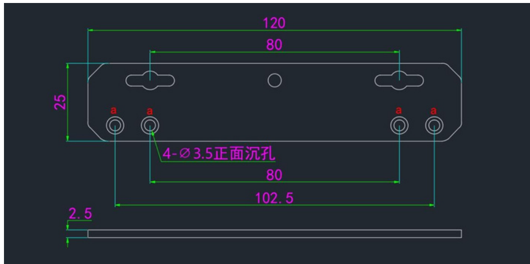
AXBOX-M342 wall mount bracket
