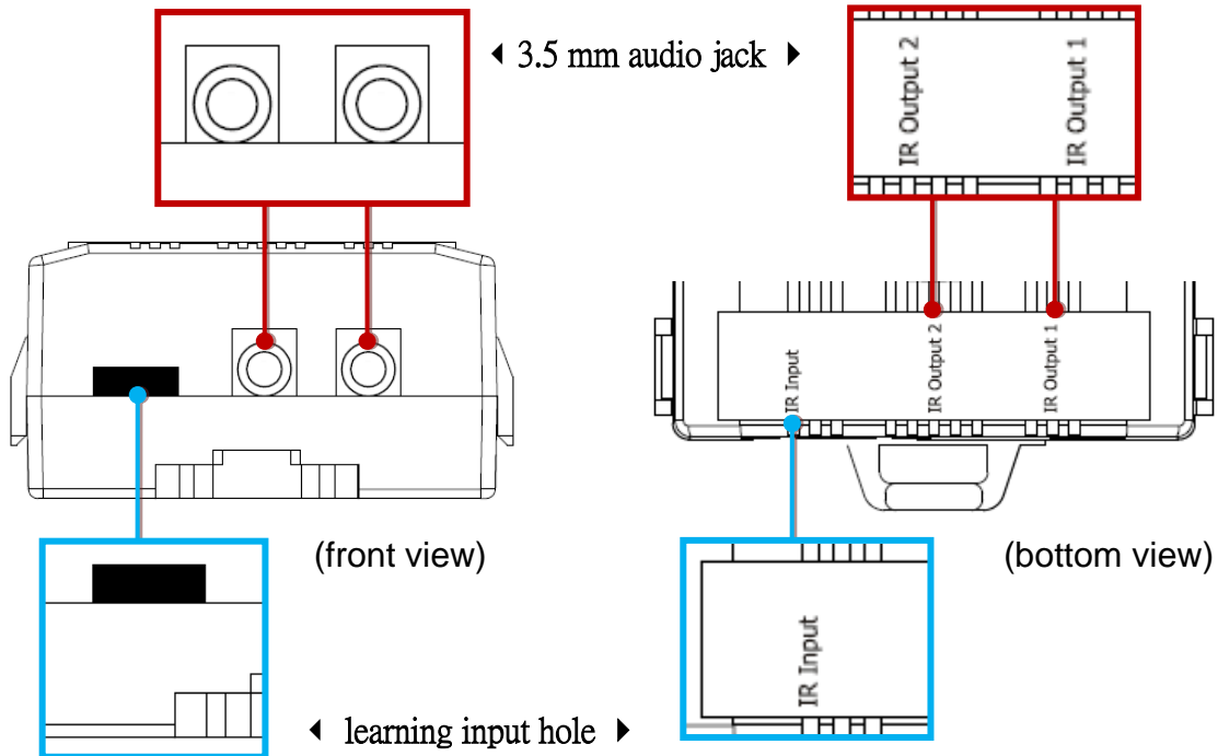
▲ Figure 2-2 IR output 3.5 mm audio jack and learning input hole
