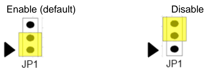
Figure 2-11 JP1 setting
